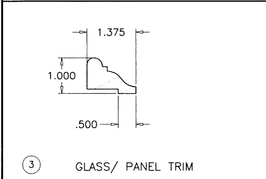
② DIRECT SET GLAZING STOP
