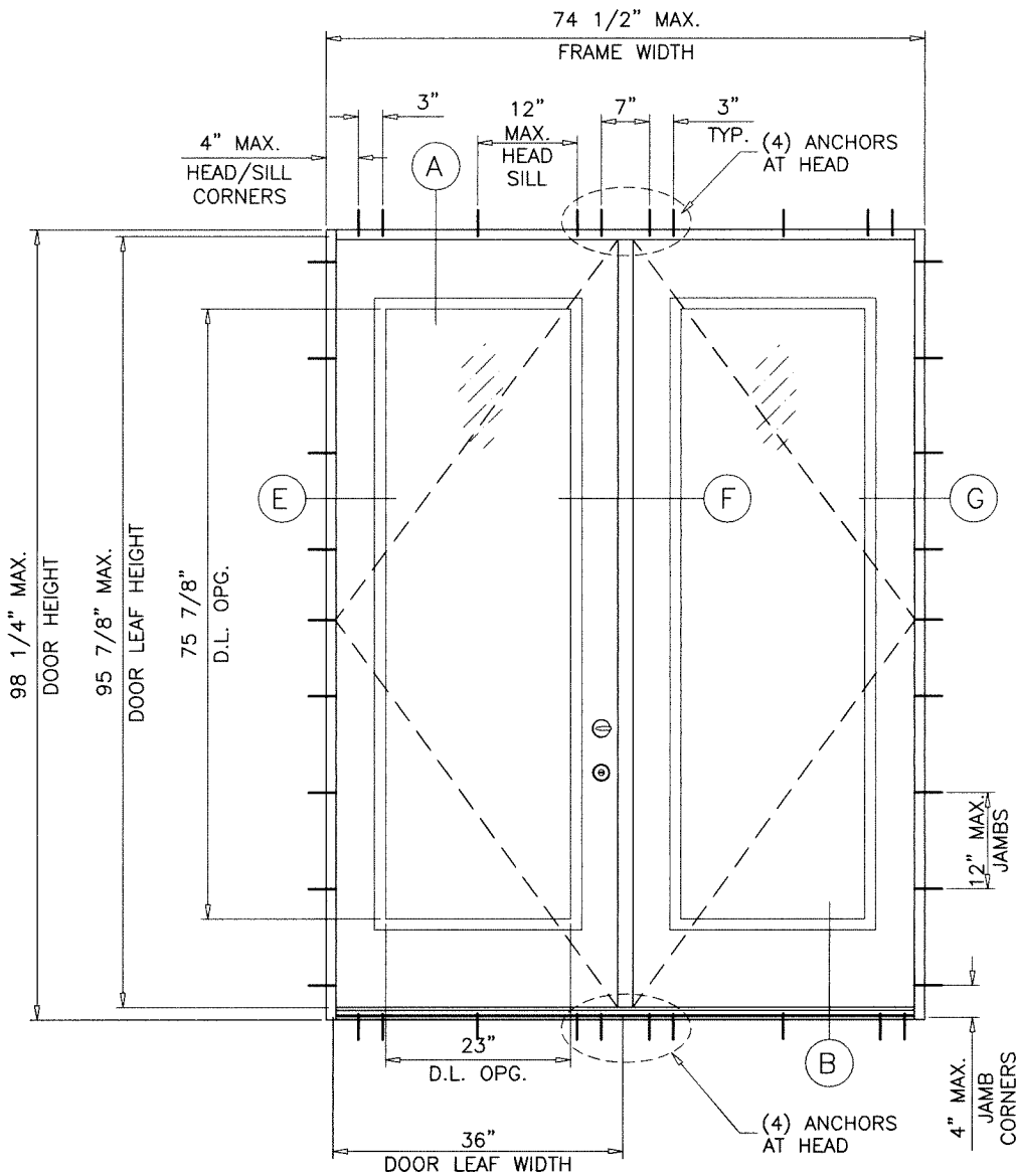
TYPICAL ELEVATION ( XX )
