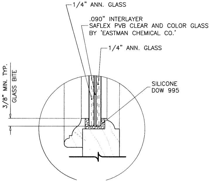
GLASS TYPE ‘1’ 9/16” OVERALL LAM. GLASS
